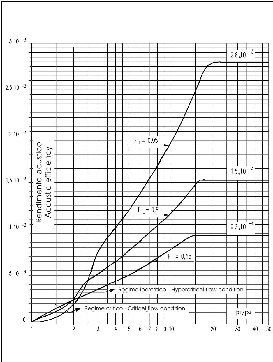
Fig. 4 Acoustic efficiency - as a function of p_1/p_2 and of F_L for \gamma = 1.3 -
