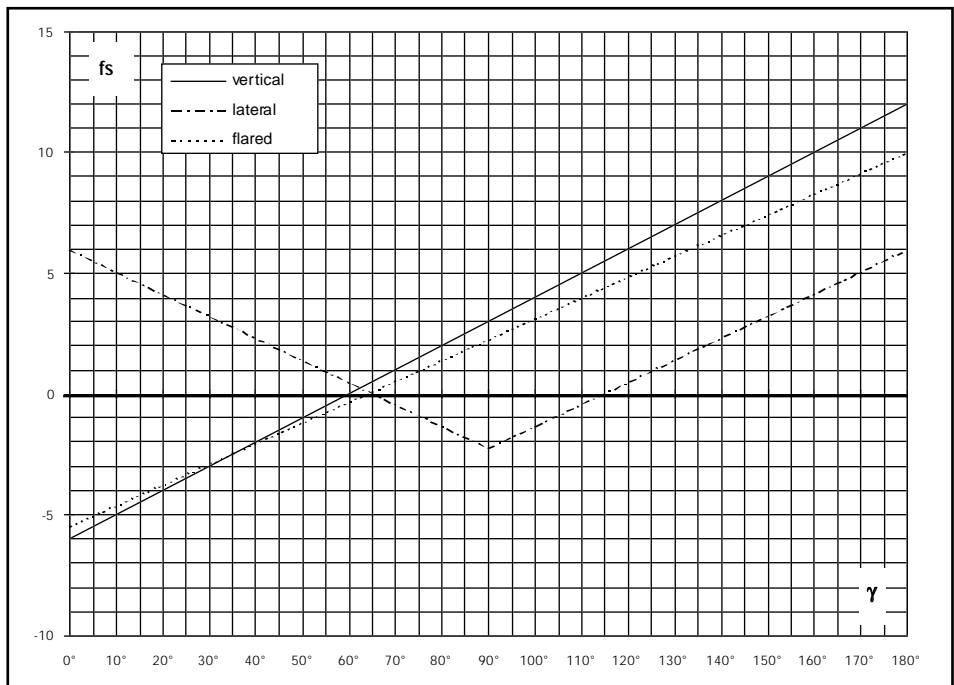
Fig. 17 Exhaust style modifier - dB
