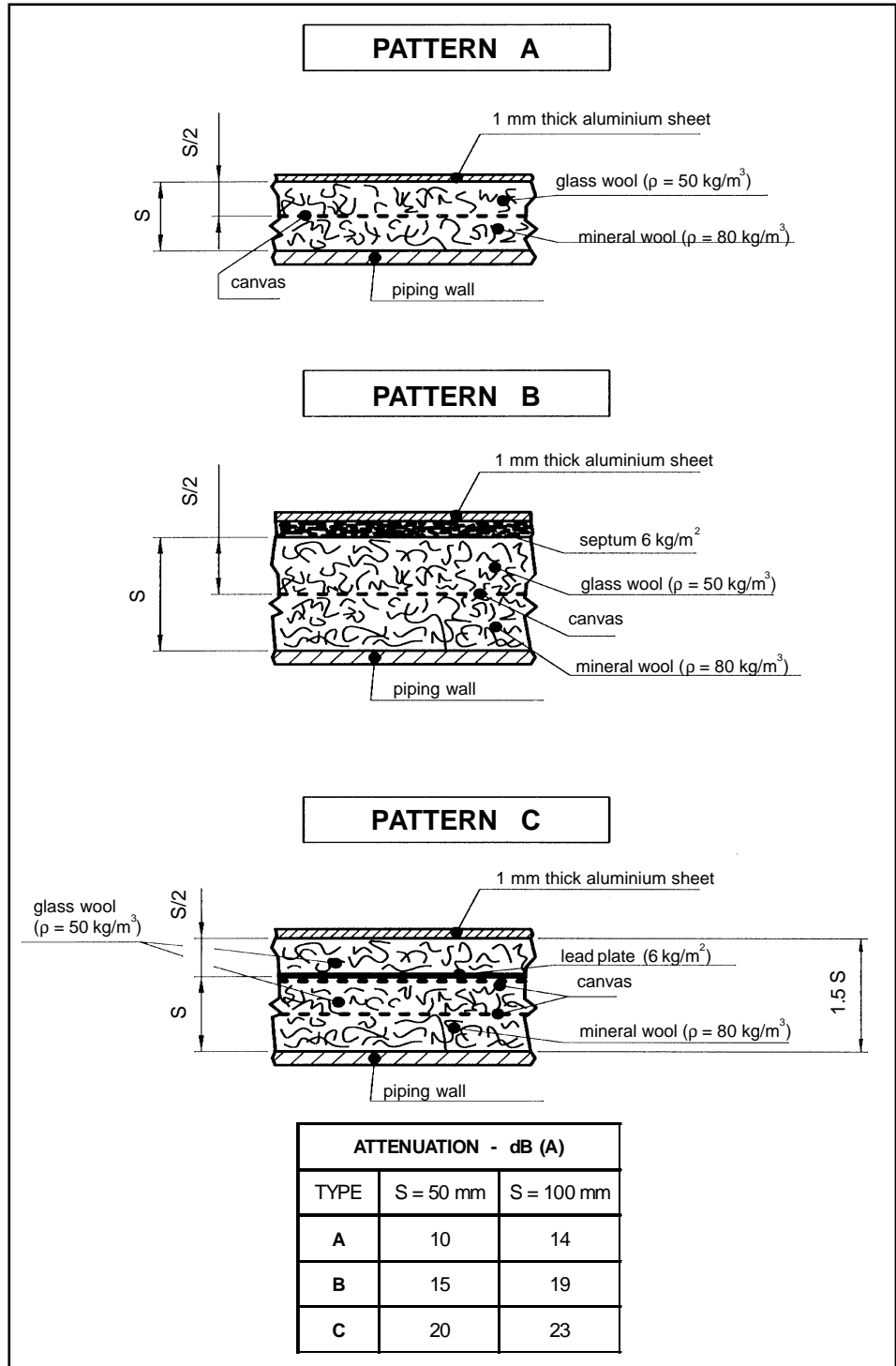
Fig. 18 Patterns of phono/thermo-insulating laggings of piping
