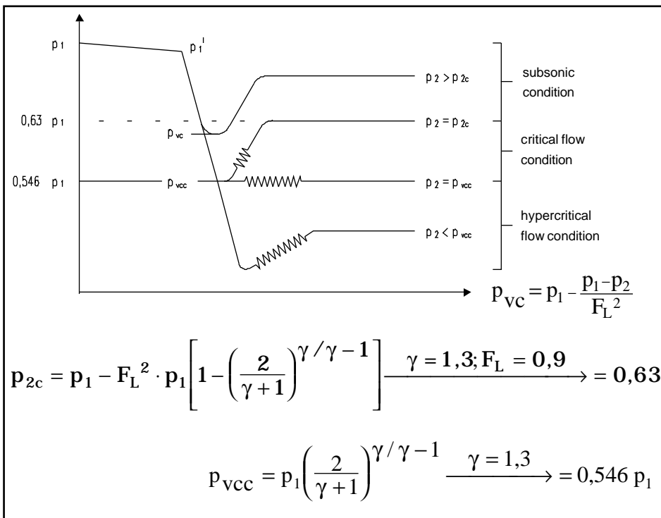
Fig. 2 Pressure run inside a single stage control valve for F_L = 0,9 servicing water steam ( \gamma = cp/cv = 1,3 , p_1 = p_1' )
