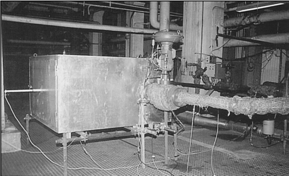
Noise test on 1-9111 Limiphon control valve DN 3" x 4" carried out on steam. Upstream pressure = 92 bar abs, upstream temperature = 485°C. Tests have been performed in accordance with IEC 534-8-1, measuring noise level in an anechoic chamber, at SIET SpA - Piacenza - ITALY
