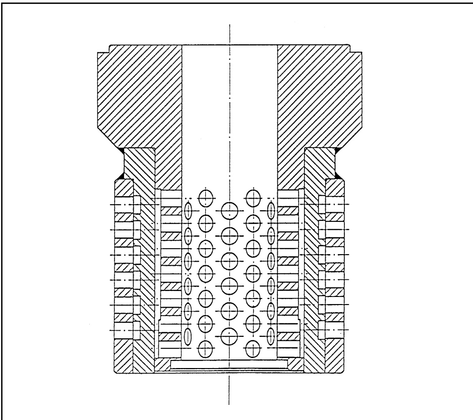
Fig. 11 Multicage trim - The limited number of stages and paths does not allow to obtain an acoustic benefit higher than 10 dB.
