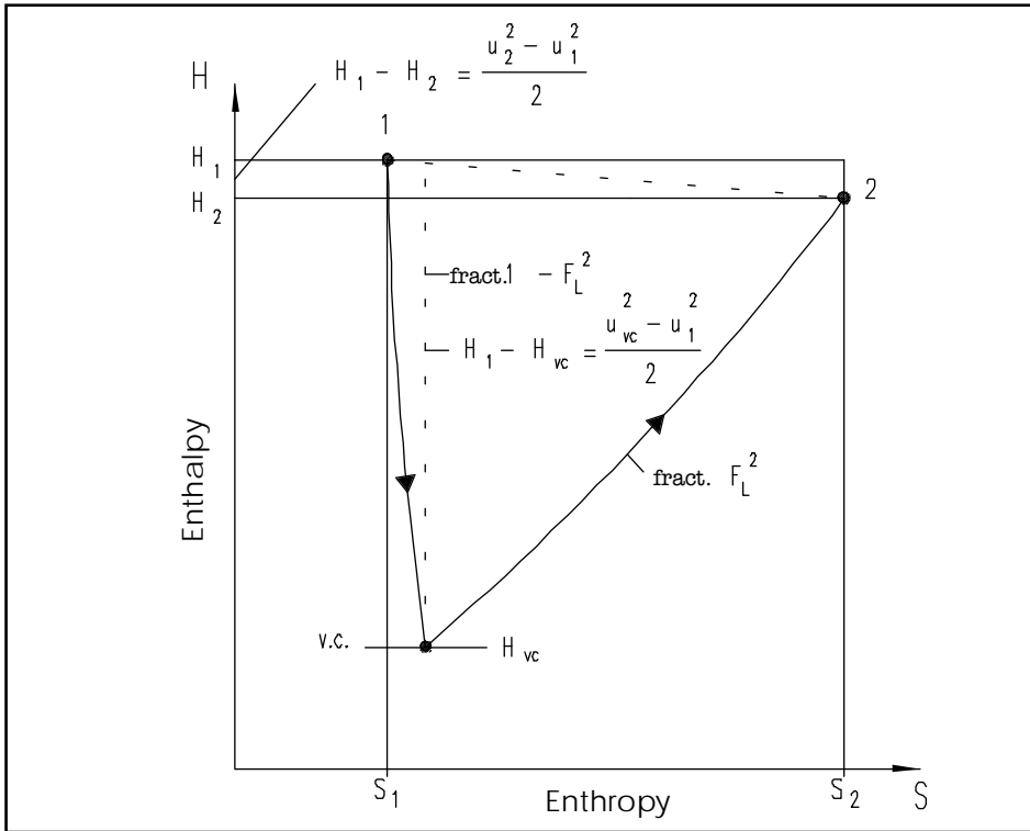
Fig. 1 Thermodynamic balance inside the valve
