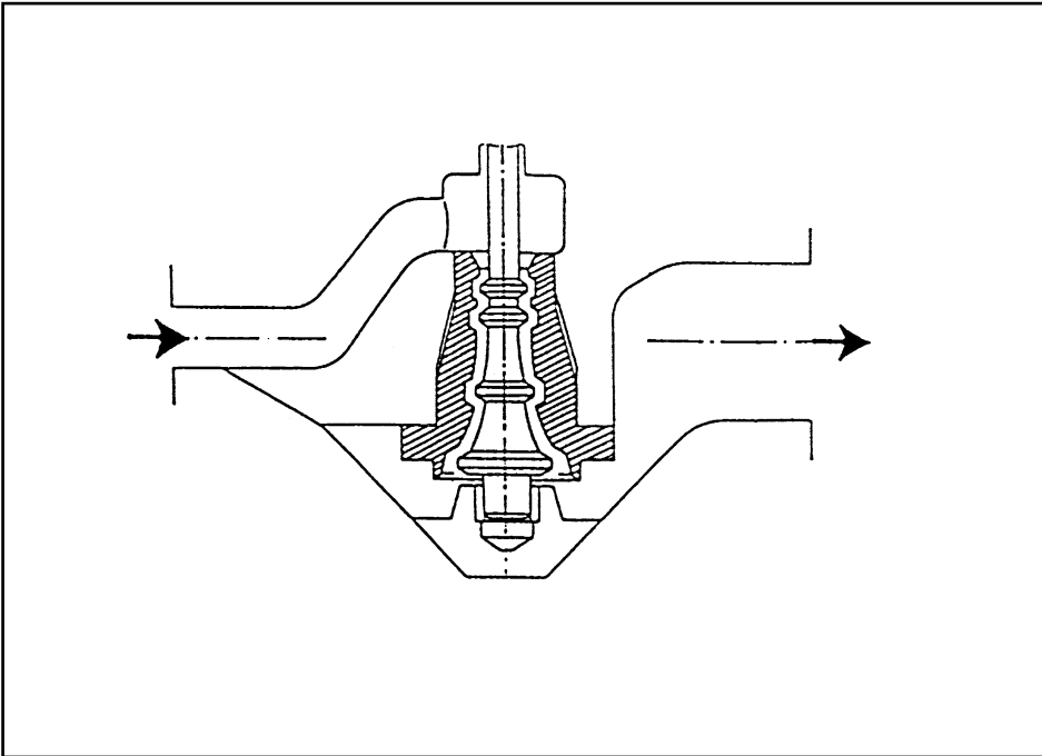
Fig. 8 Low noise design 1-7251 provided with multistage single path trim.
