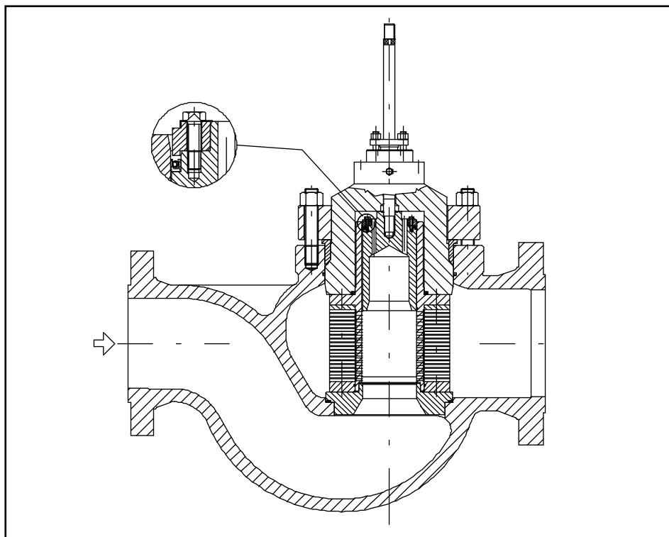
Fig. 13 Multistage/multipath low noise type reducing valve, provided with the characteristic disk stack - Model suitable for low temperature service, like stations for methane gas pressure 1st stage reduction.
