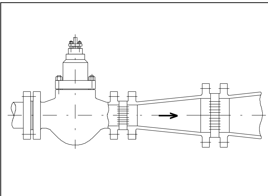
Fig. 9 Fixed downstream restrictors
