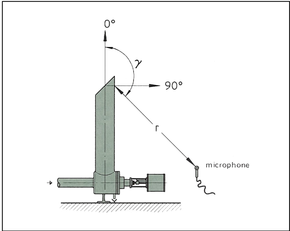
Fig. 16 Microphone distance
