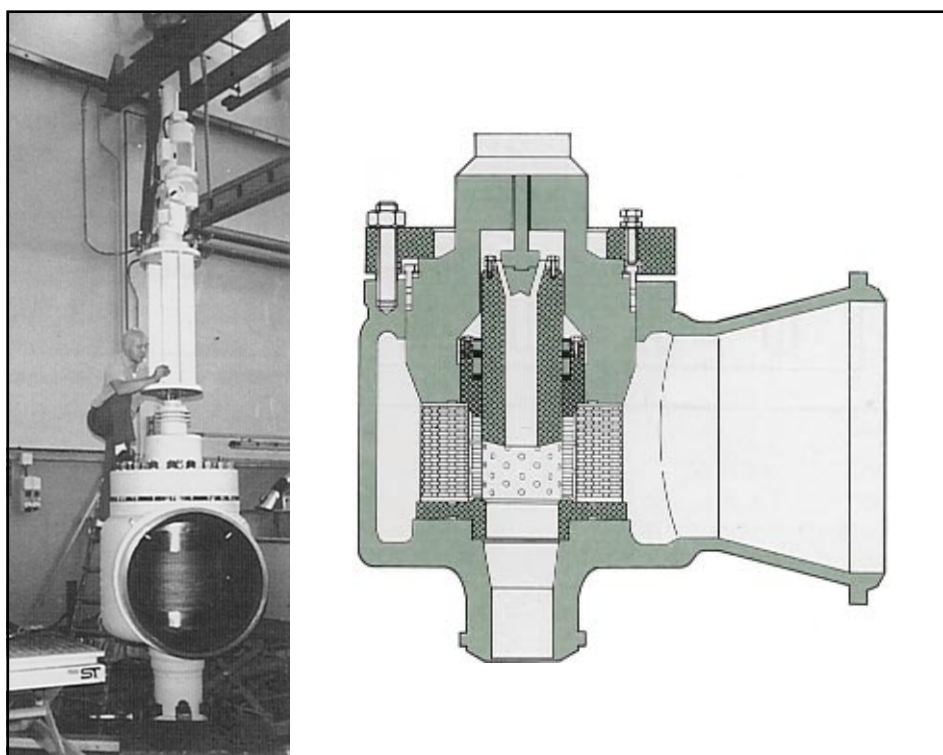
Fig. 14 Low noise model universal type suitable for service on high temperature steam - The picture shows a very exacting application: by-pass for condensation turbine DN 12" x 34" p_1 = 100 \text{ bar} - p_2 = 1.5 \text{ bar} - max steam flow rate = 250 t/h -max L_p = 90 \text{ dB(A)} (bare pipe)
